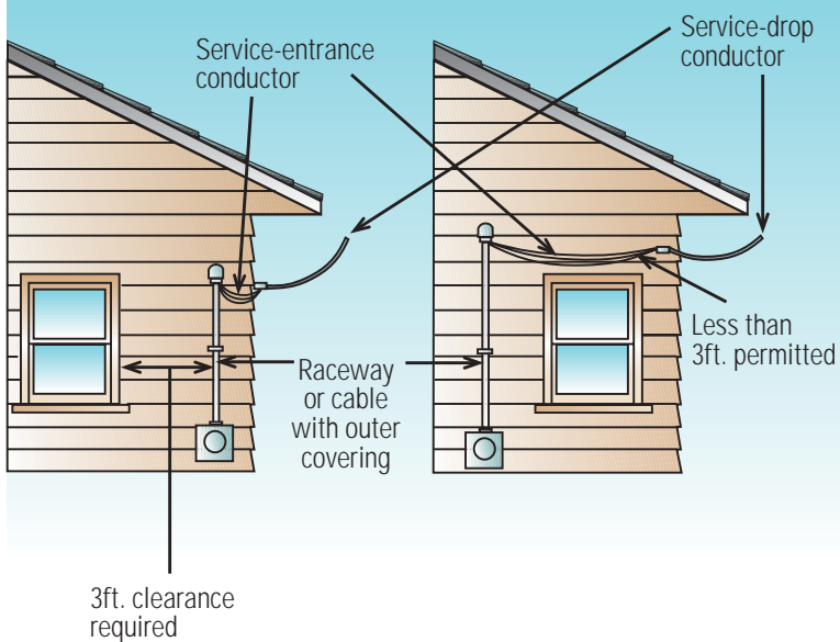
Conductors in drip loops (from type SE cables) (Courtesy NFPA)
